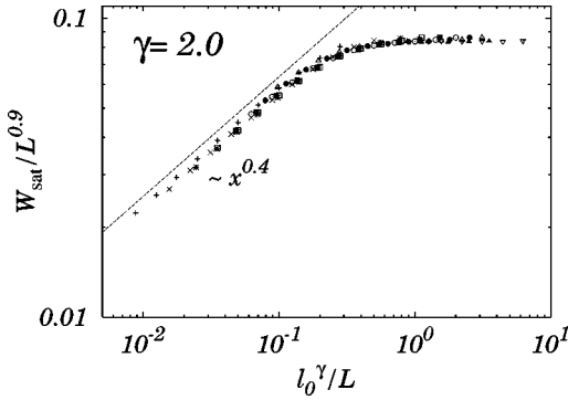
FIG. 3. Scaling plot of saturated widths of the one-dimensional RSOS/H model. The scaling variable is l_0^\gamma/L . The values of l_0 are equal to those in Fig. 2. We also draw the line x^{\alpha_{vld} - \alpha_{kpz}} = x^{0.4} as a guide to the eye.
